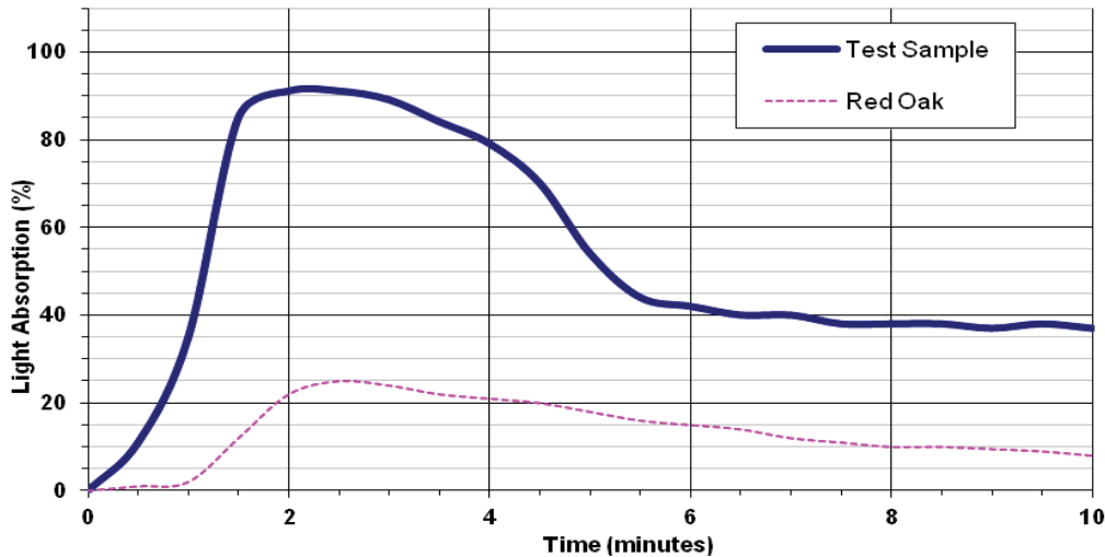
Figure 2 Smoke Developed Chart
