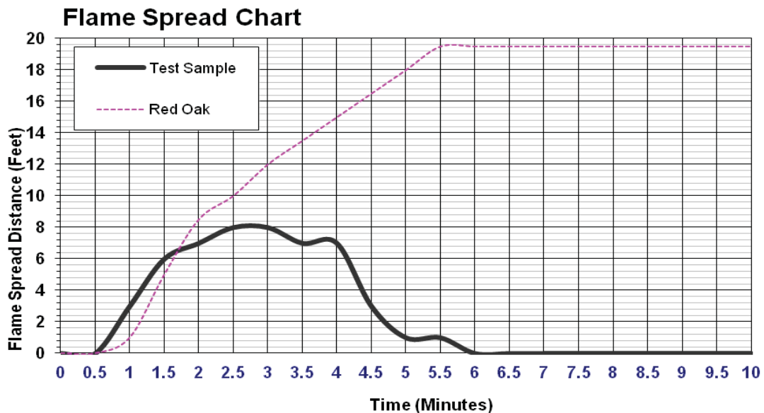
Figure 1 Flame Spread Chart
